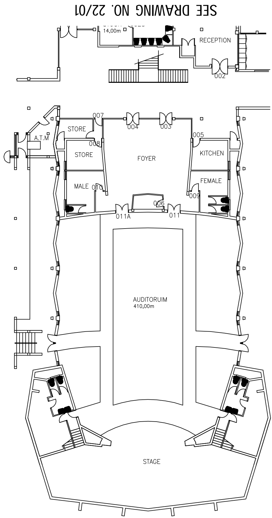
GROUND FLOOR PLAN SCALE 1:250
